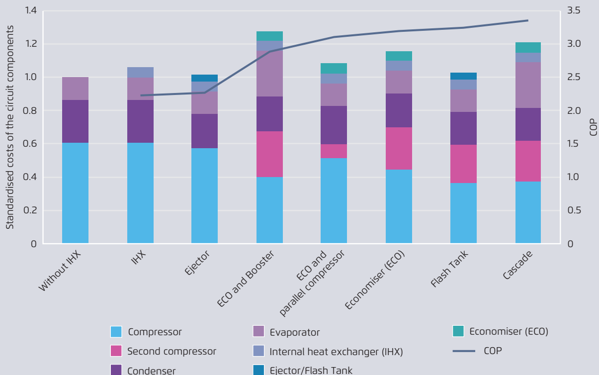
Illustrative impact of different configurations on the costs of the circuit components and the COP under constant parameters*
